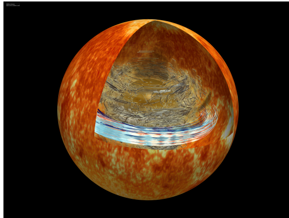
Figure 1: Turbulence and magnetic field generated in the radiative star.
